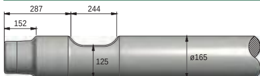
FIGURE 277 NPK E-225
