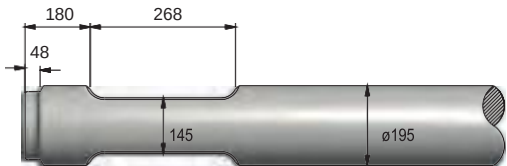
FIGURE 142 INDECO HP9000
