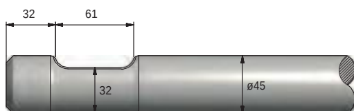
FIGURE 83 FURUKAWA F3 / FX35
