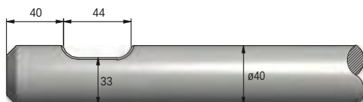
FIGURE 19 ATLAS COPCO SB100
