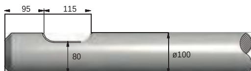
FIGURE 35 ATLAS COPCO MB750
