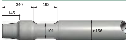
FIGURE 276 NPK E-24X / E-224
