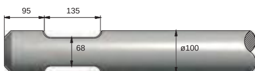
FIGURE 35 ATLAS COPCO MB750
