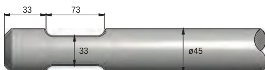
FIGURE 20 ATLAS COPCO SB102
