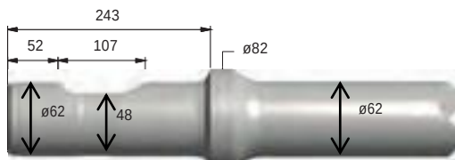
FIGURE 205 MONTABERT SILVER CLIP 22 (SC22)
