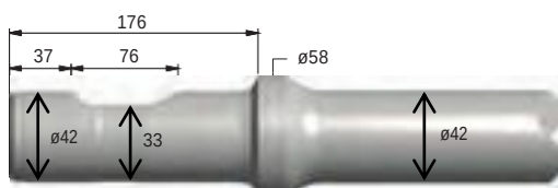
FIGURE 203 MONTABERT SILVER CLIP 12 (SC12)
