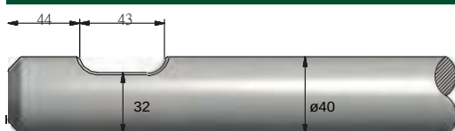
FIGURE 337 RAMMER BR255
