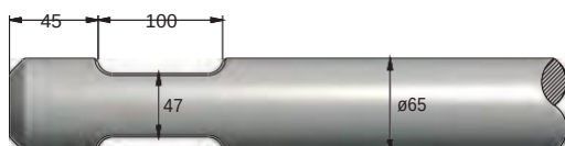
FIGURE 23 ATLAS COPCO SB300 / SB302
