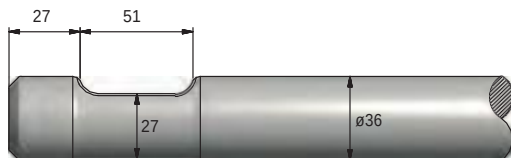
FIGURE 82 FURUKAWA F2 / HB2G / FX25
