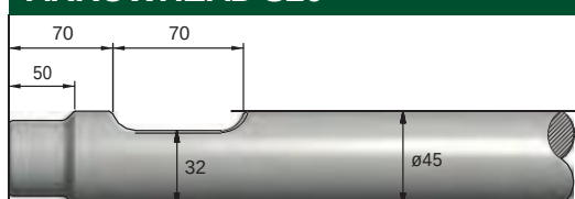
ARROWHEAD S30 (MK1 WITH COLLAR)
