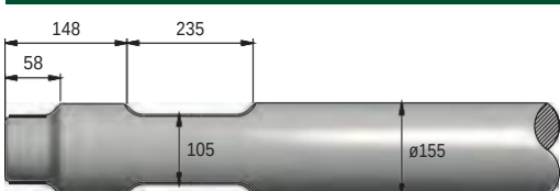
FIGURE 389 SOCOMEK MDO 2050
