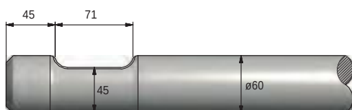
FIGURE 85 FURUKAWA F5 / FX55
