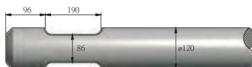
FIGURE 153 ITALDEM GK 1600
