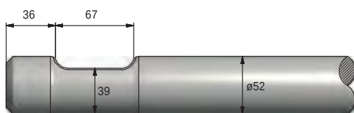
FIGURE 84 FURUKAWA F4 / FX45
