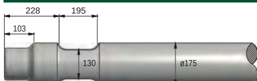
FIGURE 238 MSB MS 45AT
