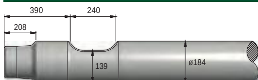
FIGURE 279 NPK E-240A
