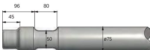
FIGURE 86 FURUKAWA F6
