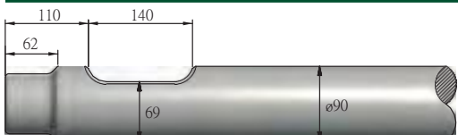
FIGURE 33 ATLAS COPCO MB500
