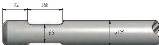
FIGURE 30 ATLAS COPCO HBC2500
