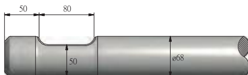
FIGURE 86 FURUKAWA F6
