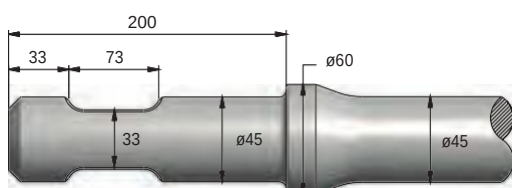
FIGURE 20 ATLAS COPCO SB102
