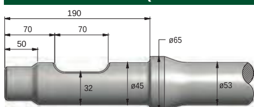
ARROWHEAD S30 (MK3)
