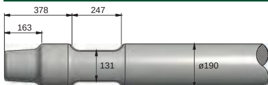
FIGURE 278 NPK E-235
