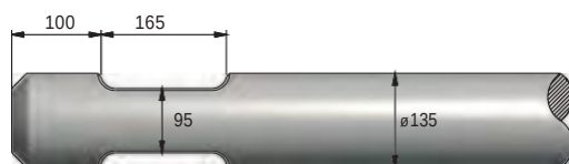
FIGURE 32 ATLAS COPCO HBC6000
