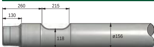
FIGURE 275 NPK E-220
