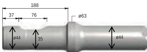
FIGURE 204 MONTABERT SILVER CLIP 16 (SC16)
