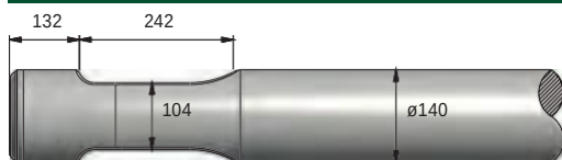
FIGURE 217 MONTABERT V1800
