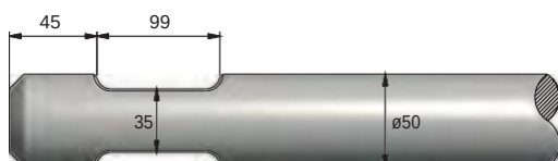
FIGURE 22 ATLAS COPCO SB200 / SB202
